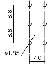
PC MOUNTING (FOR REFERENCE)
