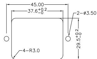
PANEL CUT-OUT
