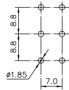
PC MOUNTING (FOR REFERENCE)
